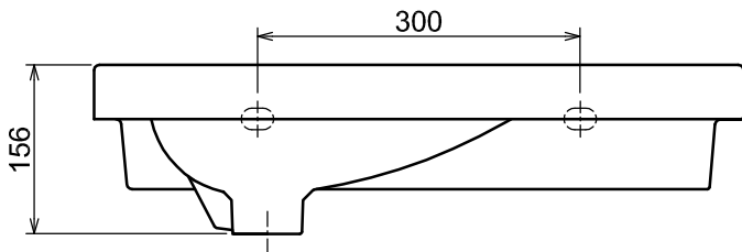
FRONT ELEVATION
