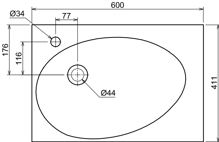
PLAN / TOP ELEVATION
