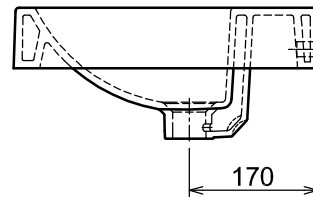
SIDE ELEVATION
